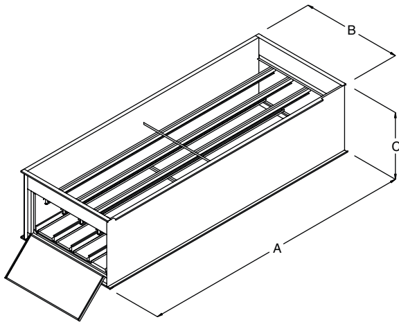
B-4000 — B-5000 UPRIGHT FILTER SECTION
