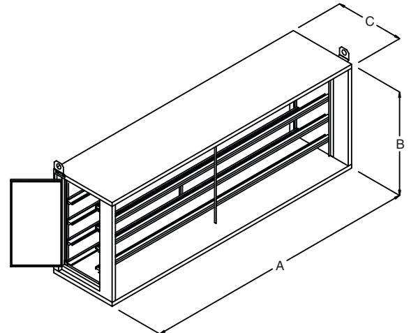
B-4000 — B-5000 HORIZONTAL FILTER SECTION
